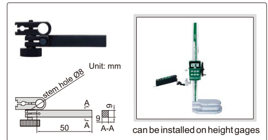
dial test indicator holder (optional)
