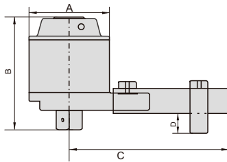
plate type
